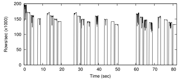
Figure 16: Rows inserted per second over time while creating the row-based TPC-H database. The discontinuities correspond to digests and combines done in the foreground.
